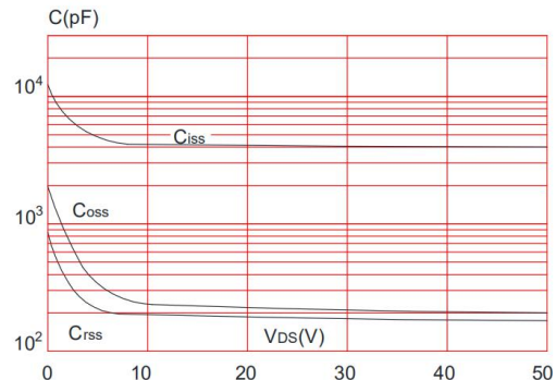
Figure 6: Capacitance Characteristics
